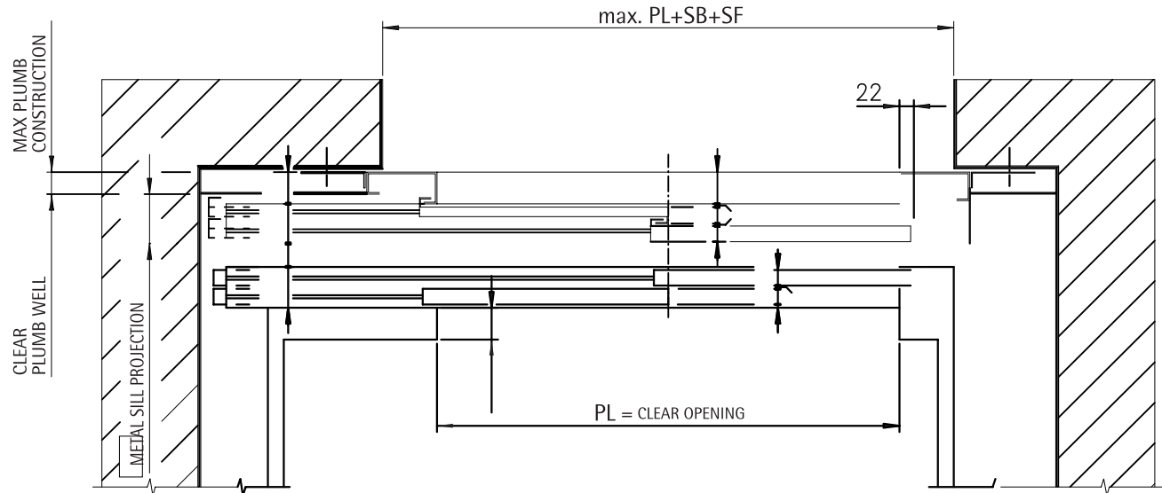
NICHE INSTALLATION
